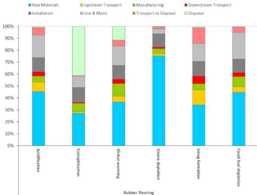
Figure 3. Contribution analysis for the flooring products – TRACI. (excluding product replacements)
