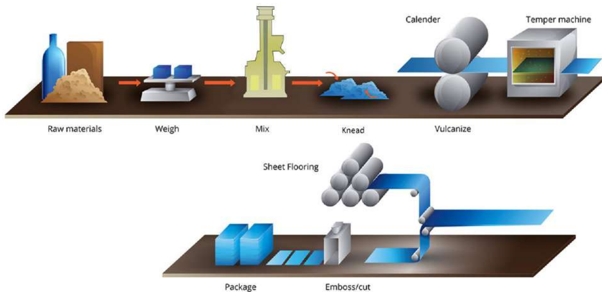
Example of Production Line for Rubber Flooring
